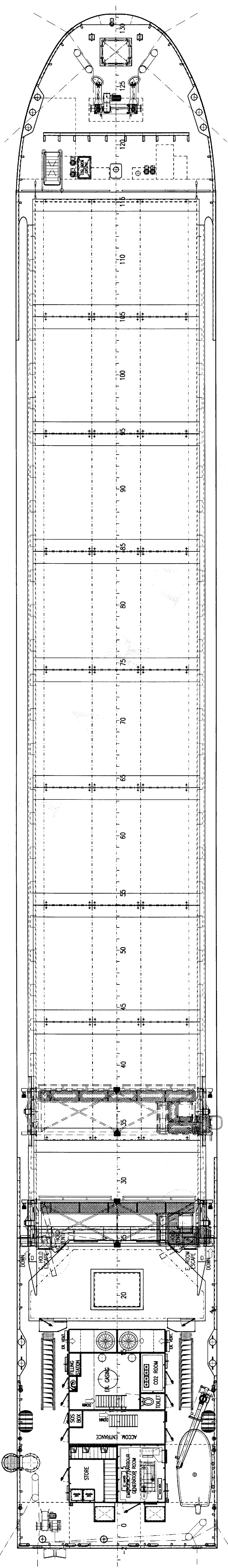
FORECASTLE DECK
